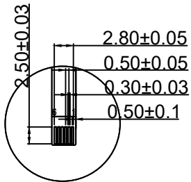
DETAIL "B" 2:1
